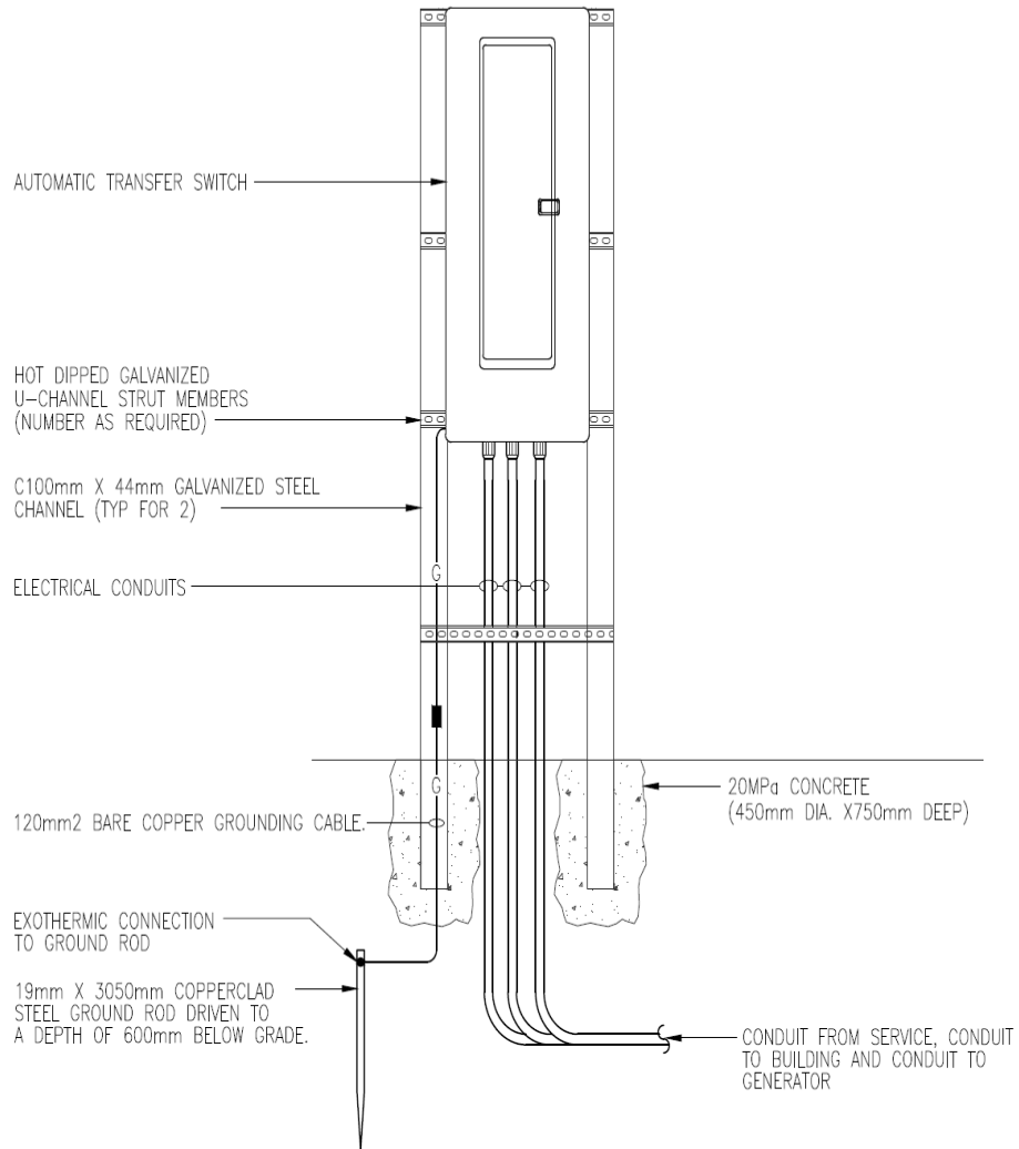
1 G9 FREESTANDING ATS SUPPORT DETAIL SCALE: NOT TO SCALE
